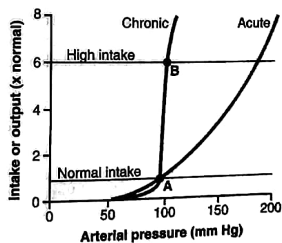
Figure 19-5 Acute and chronic renal output curves. Under steady-state conditions renal output of salt and water is equal to intake of salt and water. A and B represent the equilibrium points for long-term regulation of arterial pressure when salt intake is normal or six times normal, respectively. Because of the steepness of the chronic renal output curve, increased salt intake causes only small changes in arterial pressure. In persons with impaired kidney function, the steepness of the renal output curve may be reduced, similar to the acute curve, resulting in increased sensitivity of arterial pressure to changes in salt intake.
