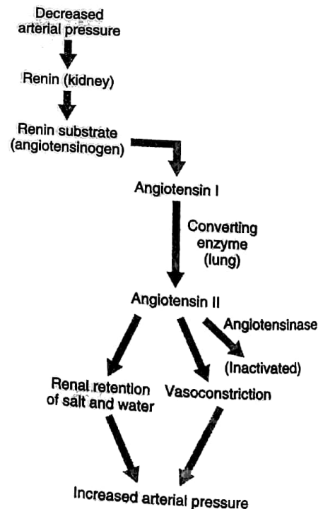
Figure 19-10 Renin-angiotensin vasoconstrictor mechanism for arterial pressure control.
