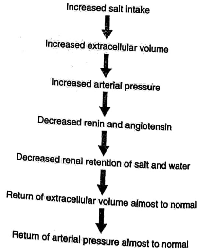
Figure 19-13 Sequential events by which increased salt intake increases the arterial pressure, but feedback decrease in activity of the renin-angiotensin system returns the arterial pressure almost to the normal level.
