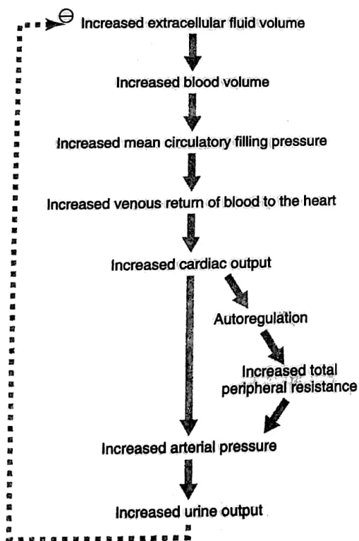
Figure 19-7 Sequential steps by which increased extracellular fluid volume increases the arterial pressure. Note especially that increased cardiac output has both a direct effect to increase arterial pressure and an indirect effect by first increasing the total peripheral resistance.
