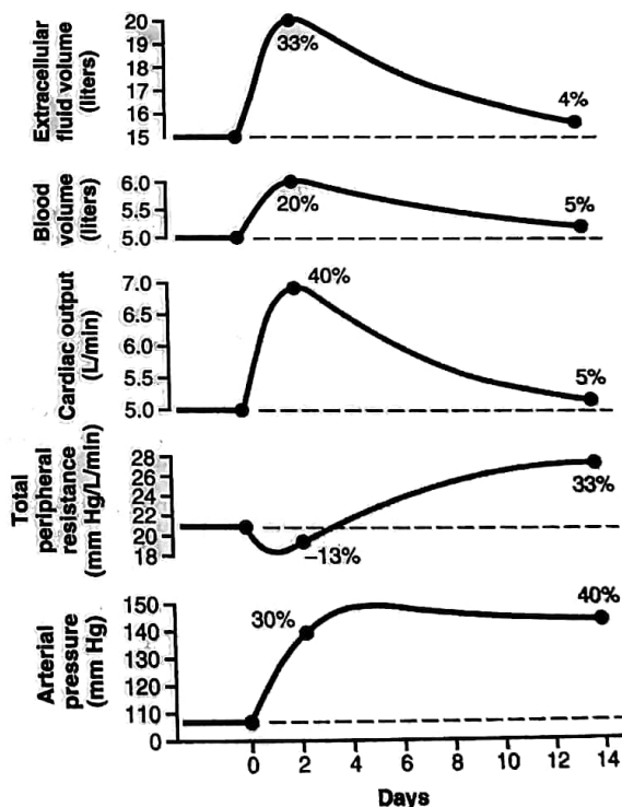
Figure 19-9 Progressive changes in important circulatory system variables during the first few weeks of volume-loading hypertension. Note especially the initial increase in cardiac output as the basic cause of the hypertension. Subsequently, the autoregulation mechanism returns the cardiac output almost to normal while simultaneously causing a secondary increase in total peripheral resistance . (Modified from Guyton AC: Arterial Pressure and Hypertension. Philadelphia: WB Saunders, 1980.)
