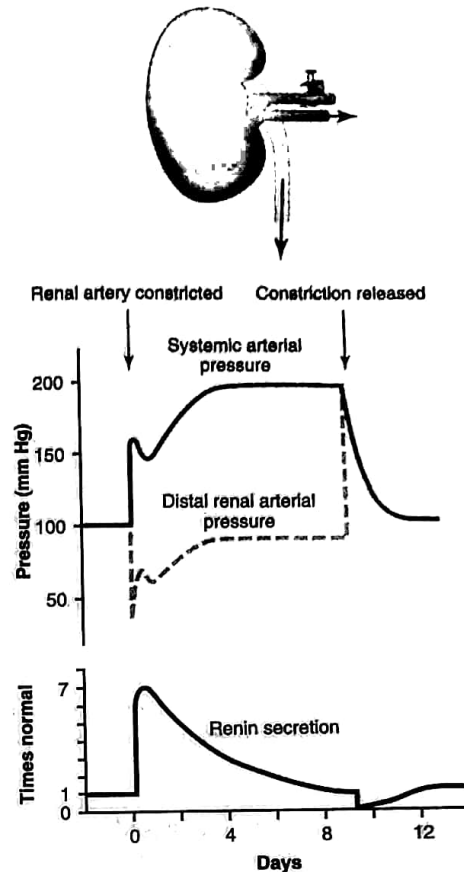
Figure 19-14 Effect of placing a constricting clamp on the renal artery of one kidney after the other kidney has been removed. Note the changes in systemic arterial pressure, renal artery pressure distal to the clamp, and rate of renin secretion. The resulting hypertension is called "one-kidney" Goldblatt hypertension.
